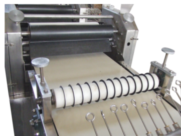
魚餃皮切條機 Fish dumpling slice cutting machine.
